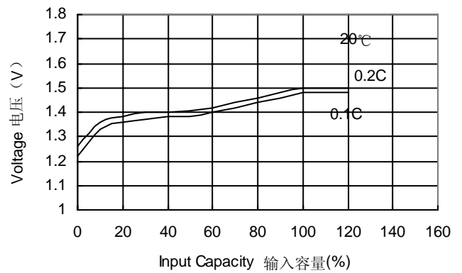
0.2C/0.1C Rate Charge Curves
