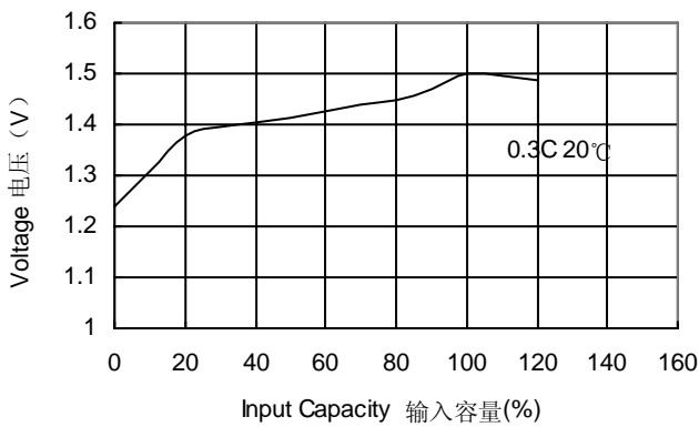
0.3C Rate Charge Curves
