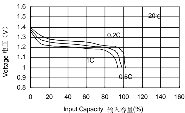
0.2C/0.5C/1C Rate Discharge Curves
