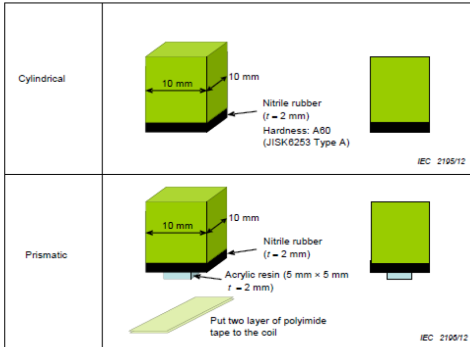
Figure 2 – Jig for pressing
