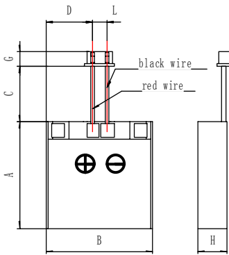
Cell adding PCB, wire
