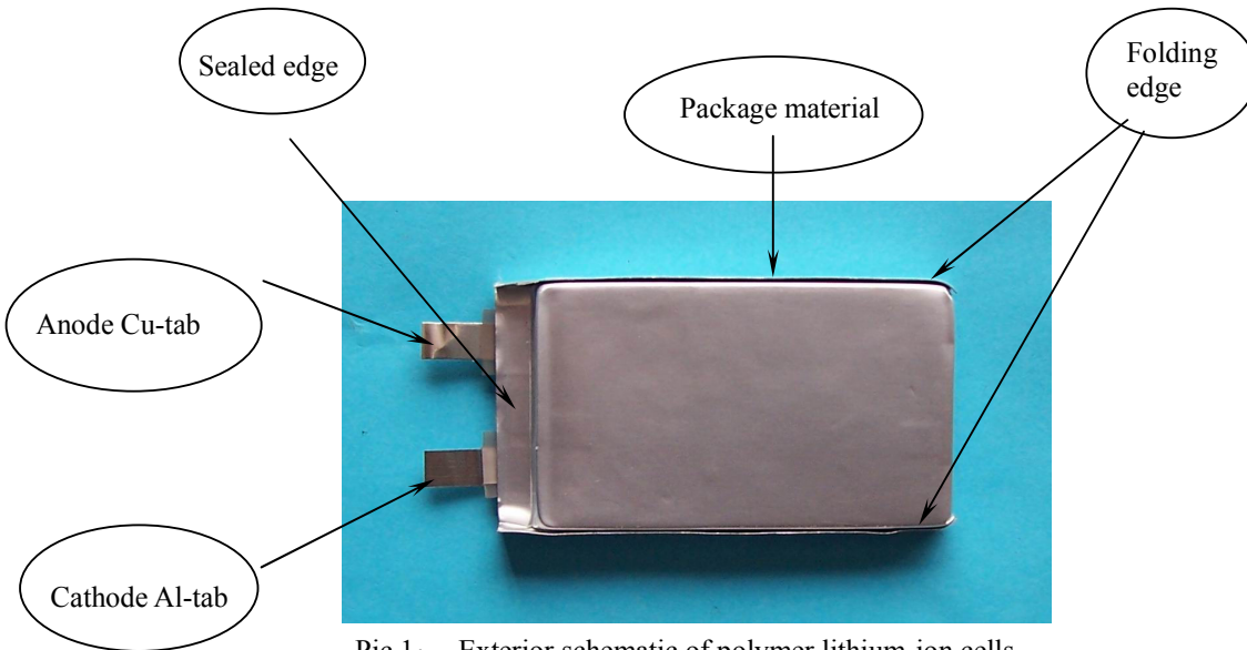
Pic 1: Exterior schematic of polymer lithium-ion cells
