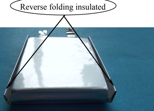
Fig.3. Reverse folding edge schematic of PL cells
