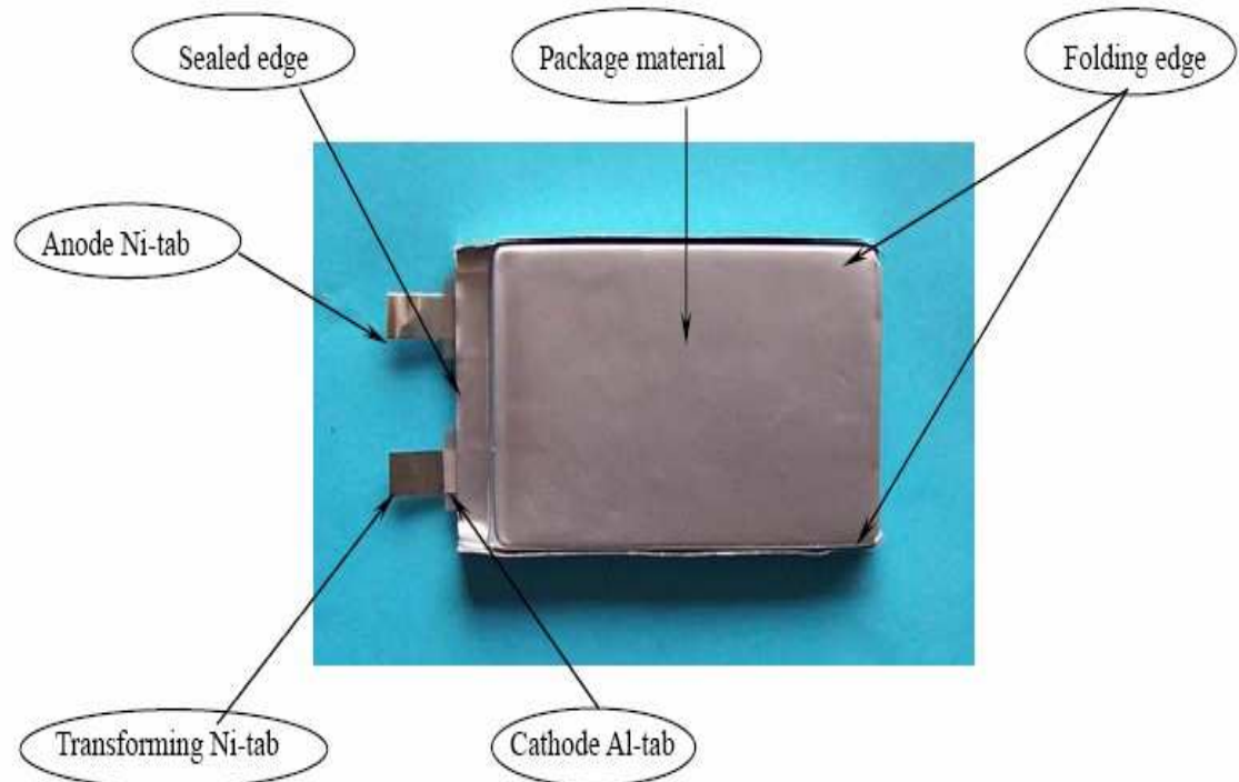
Fig.1. Exterior schematic of polymer lithium-ion cells
