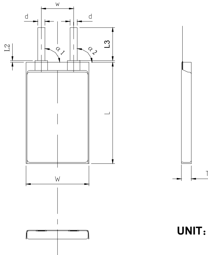
Fig.1 Dimensional Drawing of PL-75/52/146
