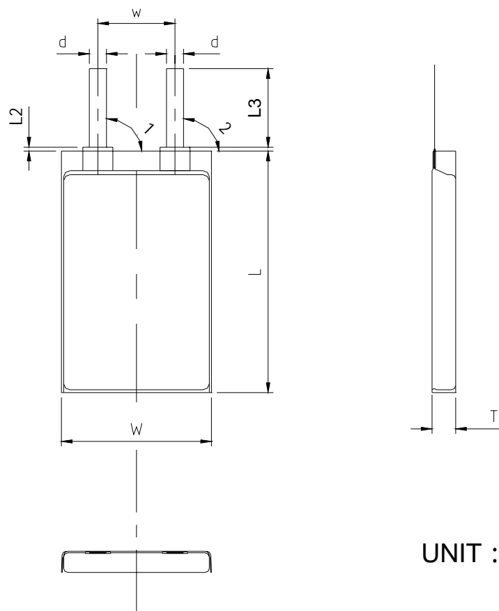
Fig.1 Dimensional Drawing of PL-355585D
